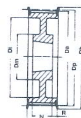
Ausf. Type 9WF
