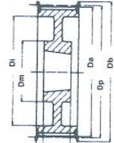
Ausf. Type 9WF
